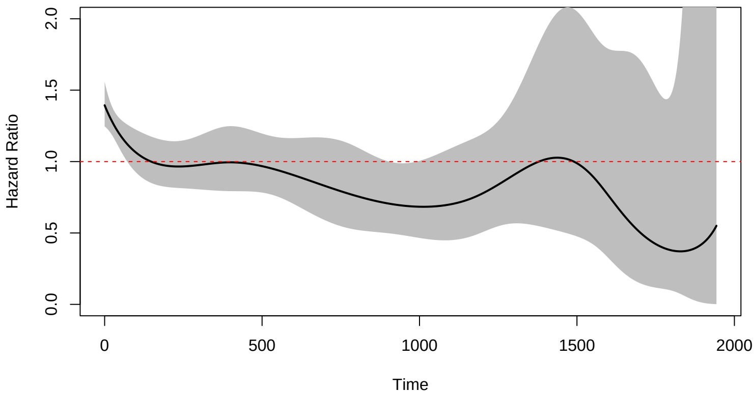
Model 7: Variable Hazard Ratio
